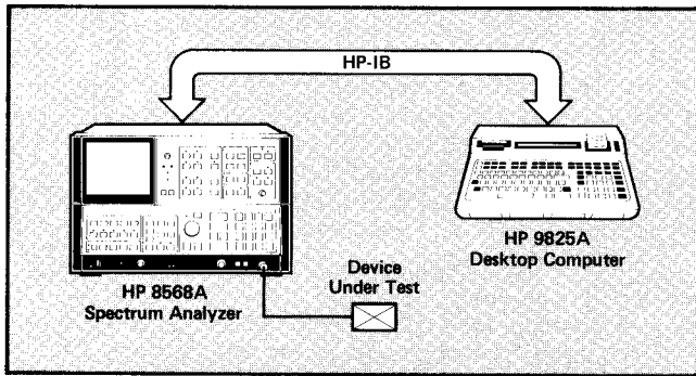
Figure 1. Measurement setup.
